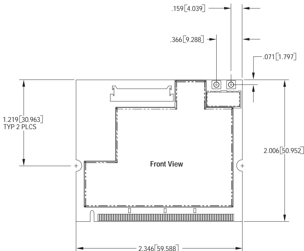
Figure 1 Cisco Aironet MPI350 Schematic
